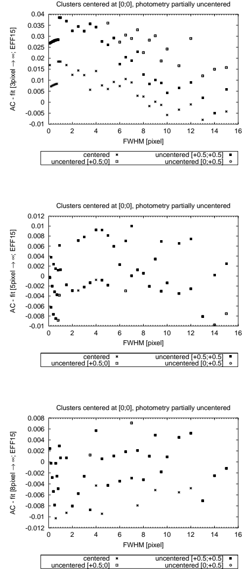
Fig. 27. ACs for clusters with annuli shifts relative to the [0;0] point, assuming a standard cluster with an EFF 15 profile. Shown are the absolute deviations between differently centered annuli with respect to the fit for the cluster at [0;0] . Top panel: AC 3 pixels \rightarrow \infty . Middle panel: AC 5 pixels \rightarrow \infty . Bottom panel: AC 8 pixels \rightarrow \infty .
