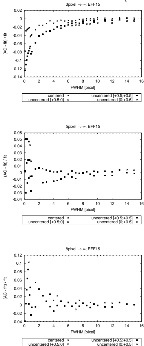
Fig. 28. ACs for clusters with annuli shifts relative to the [0;0] point, assuming a standard cluster with an EFF 15 profile. Shown are the relative deviations between differently centered annuli with respect to the fit for the cluster at [0;0] . Top panel: AC 3 pixels \rightarrow \infty . Middle panel: AC 5 pixels \rightarrow \infty . Bottom panel: AC 8 pixels \rightarrow \infty .
