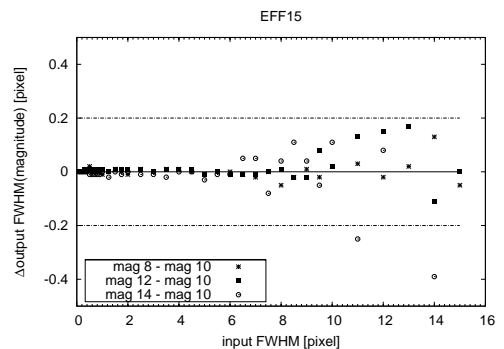
Fig. 7. Fitted Gaussian FWHM for input EFF 15 profiles of different cluster magnitudes. Top: Output – input sizes, simulated data and fitted polynomials. Bottom: Comparison of fit functions, using the V = 10 mag fit function as reference.
