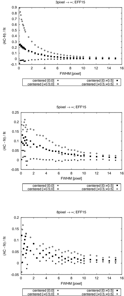
Fig. 26. ACs for clusters with subpixel shifts relative to the [0;0] point, assuming a standard cluster with an EFF 15 profile. Shown are the relative deviations between differently centered clusters with respect to the fit for the cluster at [0;0] . Top panel: AC 3 pixels \rightarrow \infty . Middle panel: AC 5 pixels \rightarrow \infty . Bottom panel: AC 8 pixels \rightarrow \infty .
