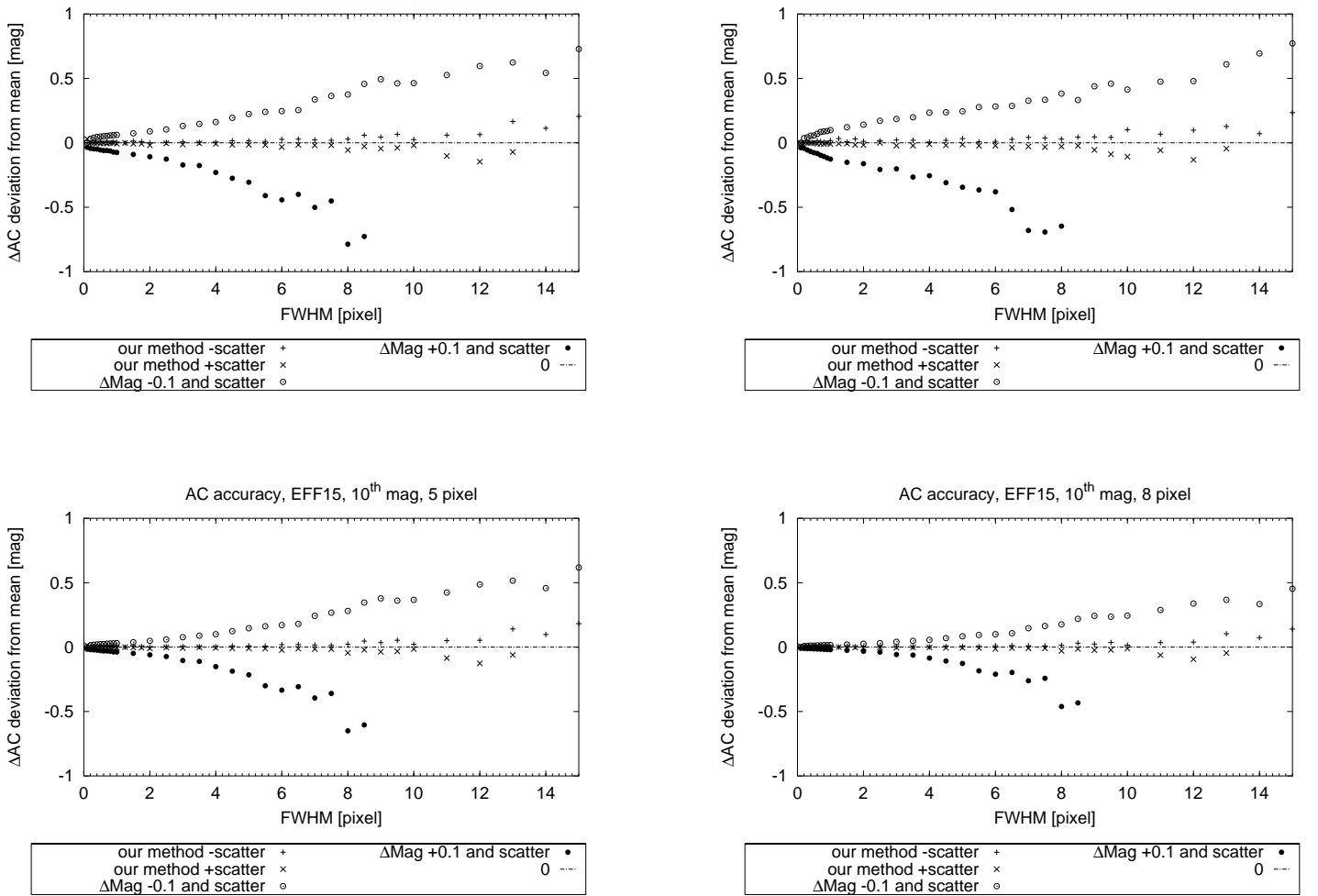
Fig. 32. Scatter in the AC calculation from the DeltaMag method (assuming a photometric accuracy of \pm 0.1 mag), compared to the scatter introduced by our method for a standard cluster. Top panels: 3 pixel radius apertures for an EFF 15 profile (left) and a King 30 profile (right). Bottom panels: Assuming an EFF 15 profile, and using 5 pixel (left) and 8 pixel (right) radius apertures.
