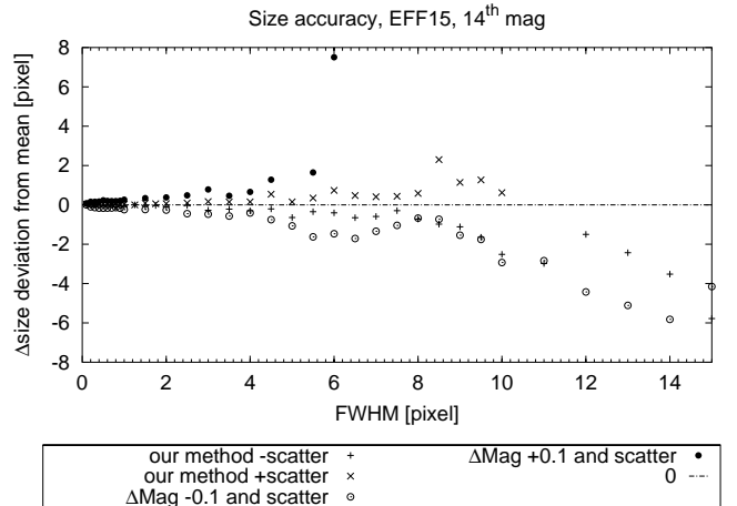
Fig. 31. Scatter in the size determination from the DeltaMag method (assuming a photometric accuracy of \pm 0.1 mag), compared to the scatter introduced by our method for a V = 14 mag cluster. Top panel: King 30 profile. Bottom panel: EFF 15 profile.
