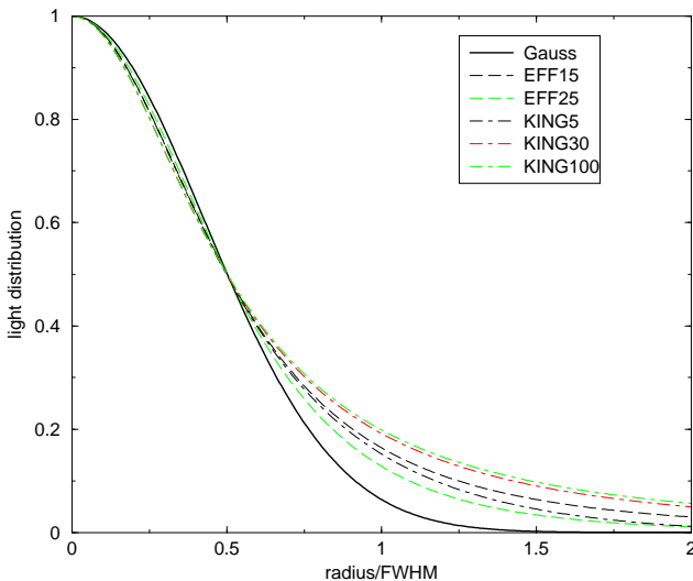
Fig. 2. Model light distributions.
