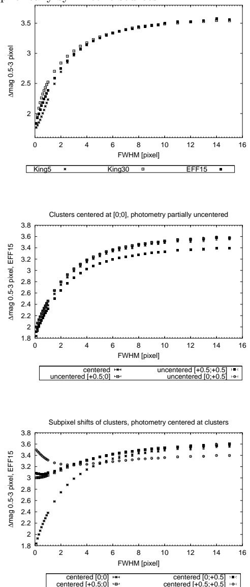
Fig. 29. Top panel: \Delta mag between 0.5 and 3 pixels, for 3 different profiles. Middle panel: Comparison of \Delta mag for off-centered aperture annuli for the EFF 15 profile. Bottom panel: Comparison of \Delta mag for different centerings of clusters on a pixel, using an EFF 15 profile.
